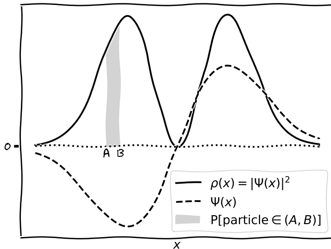
Fig. 1: Wave function (dashed line) and probability density (solid line). The probability that a particle occurs somewhere between a and B is then the area of the grey-shaded region.
